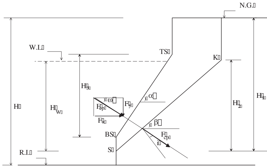
Figure 5. Parameters of hydrostatic confining force and failure plane angle using the Stability approach.
