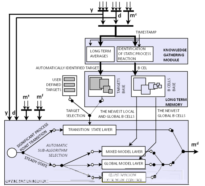
Fig. 2. Optimization and Knowledge Gathering module.
